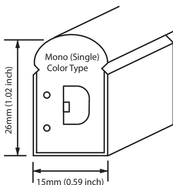
For Mono (Single) color LED Rainbow Flex will have 2 Pins
