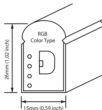
For RGB color LED Rainbow Flex will have 4 Pins
